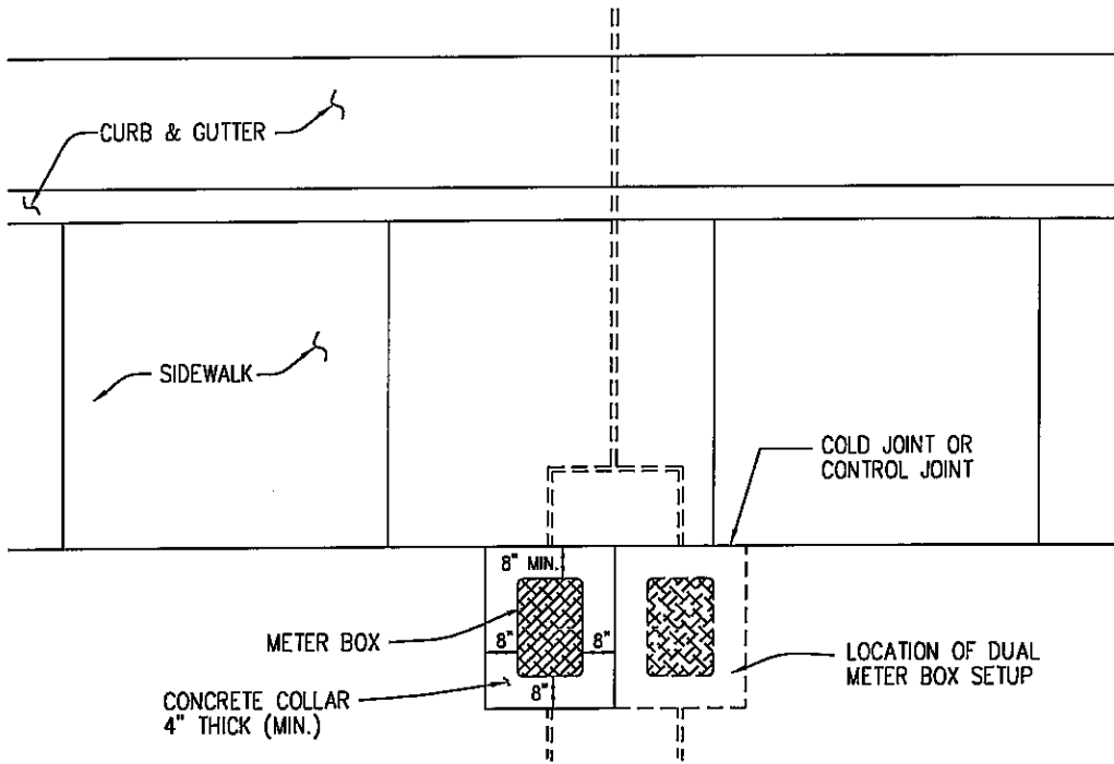
PLAN VIEW W/SIDEWALK
