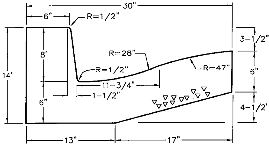
STANDARD CURB & GUTTER (TYPE HB30-8)
