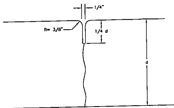
CONTROL JOINT
