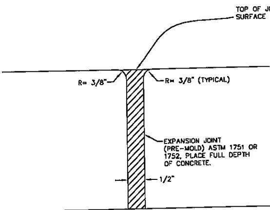
EXPANSION JOINT
