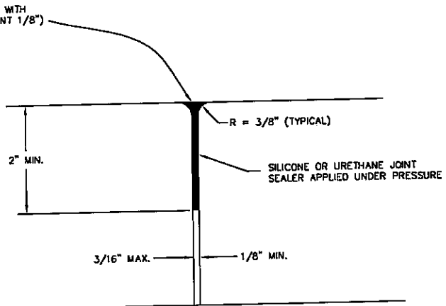
FORM PLATE JOINT
