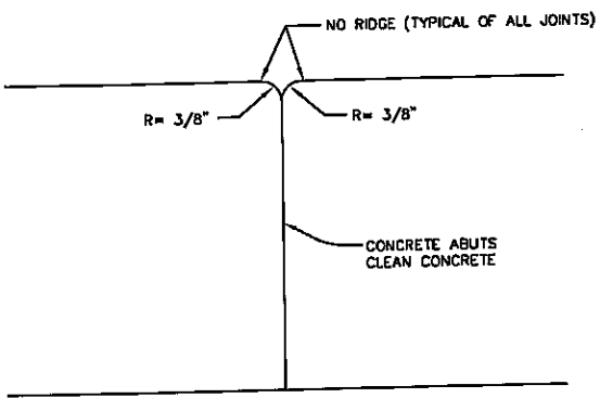
COLD JOINT
